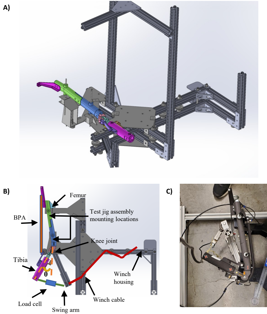
Figure 3.2: (A) CAD solid model assembly of the revolute joint knee in the test stand. (B) 1-DoF pinned-joint robot knee in the test apparatus with important components labeled. Leg is shown with 30 degrees flexion, i.e. \theta_k = -30^\circ . (C) Picture from isometric torque testing. Setup shows the revolute knee configured for a test of the extensor BPA. The knee is flexed with \theta_k = -120^\circ . Also note the compressed shape of the inflated BPA on the knee during this high degree of flexion.
