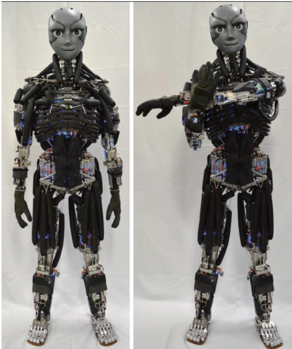
Figure 2.1: Kengoro human-mimetic musculoskeletal humanoid in neutral and upper-limb poses, illustrating its human-scale skeletal structure and densely routed tendon-driven musculature [Asano et al., 2017].
