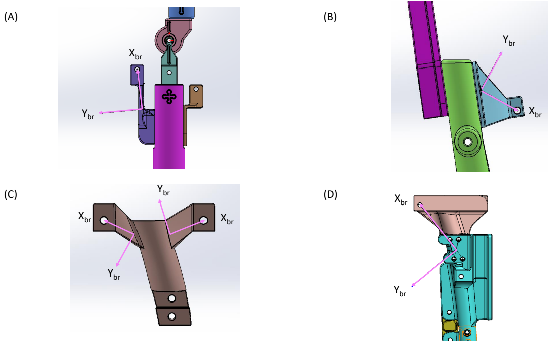
Figure 3.5: Bracket frame orientations for: (A) flexor configuration on the pinned knee, (B) extensor configuration on the pinned knee, (C) flexor and extensor configurations on the biomimetic knee with \phi 10 mm BPAs, and (D) flexor configuration on the biomimetic knee with the \phi 20 mm BPA.
