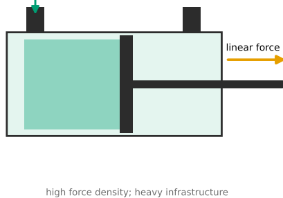
Figure 2.2: Representative operating mechanisms for robotic actuators. (A) An electric torque motor produces controlled shaft rotation. (B) A braided pneumatic actuator shortens as internal pressure expands its sleeve radially. (C) A hydraulic cylinder converts fluid pressure into linear piston force. (D) A dielectric elastomer thins and expands laterally under an applied electric field. The panels use a consistent schematic style to emphasize the distinct energy-conversion mechanisms and design tradeoffs summarized in the text [Suzumori and Faudzi, 2018, Liang et al., 2020].
