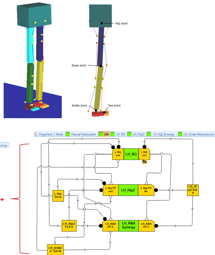
Figure 3.8: AnimatLab model and architecture illustrations. Top: the segmented walker and labeled hip, knee, ankle, and toe joints. Bottom: the left/right subsystem organization and an expanded view of the left-side rhythm-generator, hip, and knee–ankle modules. These architectural views describe model organization and are not snapshots of the phase-1 trajectory.
