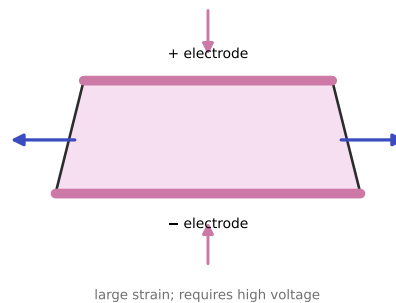
Figure 2.2: Representative operating mechanisms for robotic actuators. (A) An electric torque motor produces controlled shaft rotation. (B) A braided pneumatic actuator shortens as internal pressure expands its sleeve radially. (C) A hydraulic cylinder converts fluid pressure into linear piston force. (D) A dielectric elastomer thins and expands laterally under an applied electric field. The panels use a consistent schematic style to emphasize the distinct energy-conversion mechanisms and design tradeoffs summarized in the text [Suzumori and Faudzi, 2018, Liang et al., 2020].
