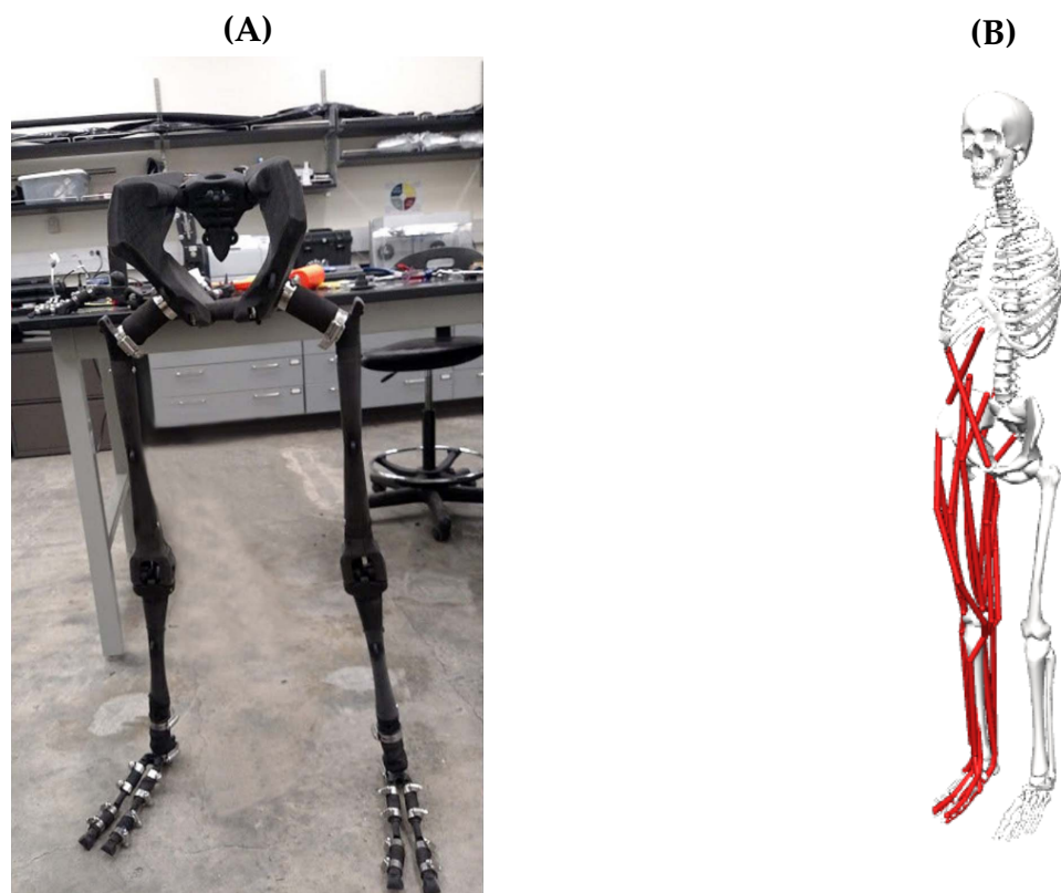
Figure 2.5: (A) The laboratory bipedal skeleton (actuators not installed in this view). (B) The Gait2392-derived OpenSim model used to develop its muscle routing; the view exposes the retained lower-limb musculotendon paths used as biomechanical design references [Bolen and Hunt, 2019, Morrow et al., 2020].
