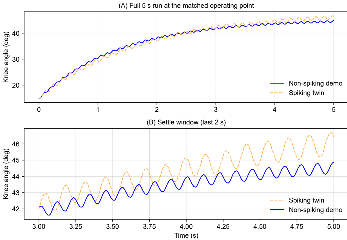
Figure 4.13: Knee angle of the Simulink knee-reflex demonstration: committed non-spiking baseline (solid indigo) versus spiking twin (dashed orange) at the matched operating point. (A) Full 5 s run. (B) Settle window (last 2 s); the spiking twin's alternation band is slightly wider.
