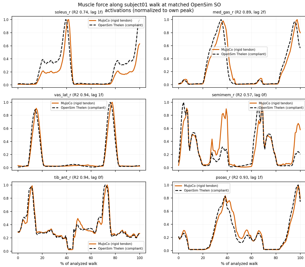
Figure A1: Normalized muscle force along the analyzed walk at matched OpenSim static-optimization activations (MuJoCo: rigid tendon; OpenSim: Thelen compliant tendon). Soleus illustrates the signature of the missing series compliance: OpenSim force is carried through mid-stance by tendon stretch while MuJoCo force follows the activation.
