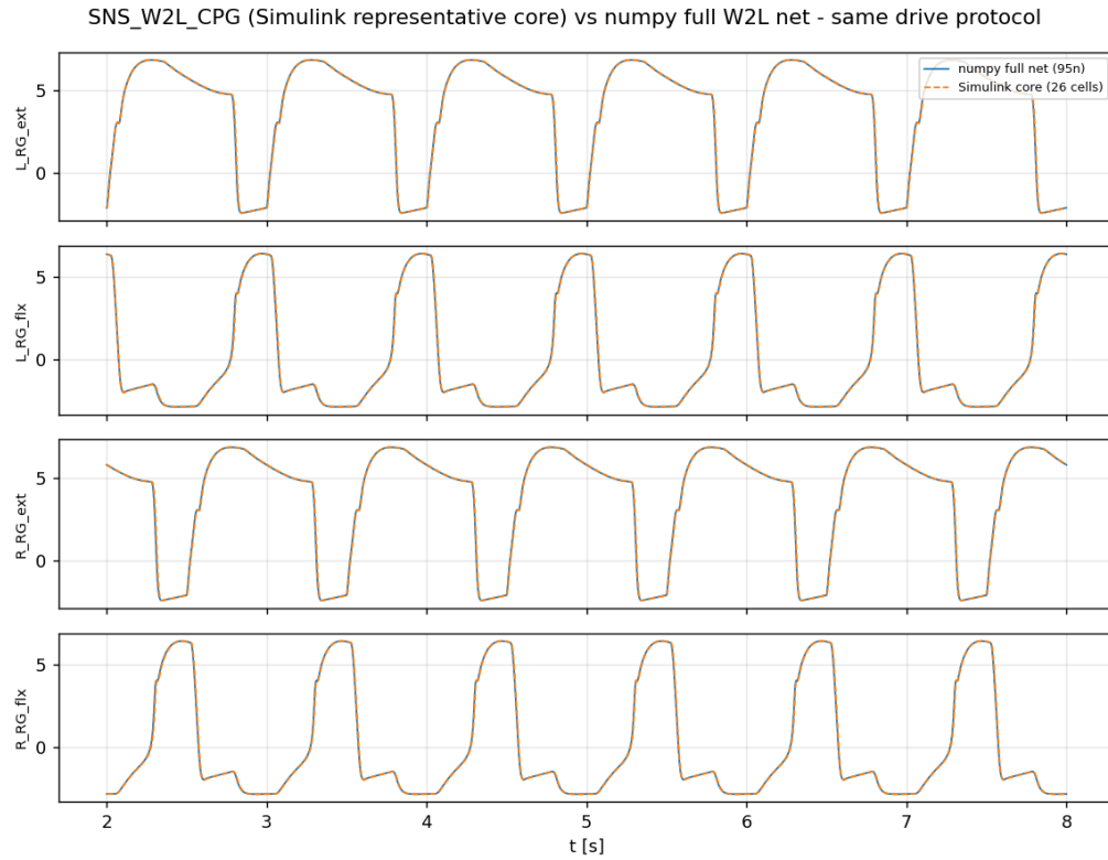
Figure 4.10: Left and right rhythm-generator extensor half-center voltages of the W2L contact-driven rhythm core under the shared verification protocol, from the NumPy reference (SNS-Toolbox backend) and the native Simulink reimplement. Scored metrics — burst period, left-right antiphase correlation, and burst counts — agree exactly, and the full traces cross-correlate at r \geq 0.99996 at a -2 ms lag.
