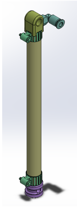
Figure 2.3: CAD representation of a Festo DMSP braided pneumatic actuator with the mounting and pneumatic connections used in the laboratory assembly [Festo AG & Co. KG, 2026]. The long cylindrical body contains the bladder and braided sleeve; pressurization through the end fittings converts radial expansion into axial contraction.
