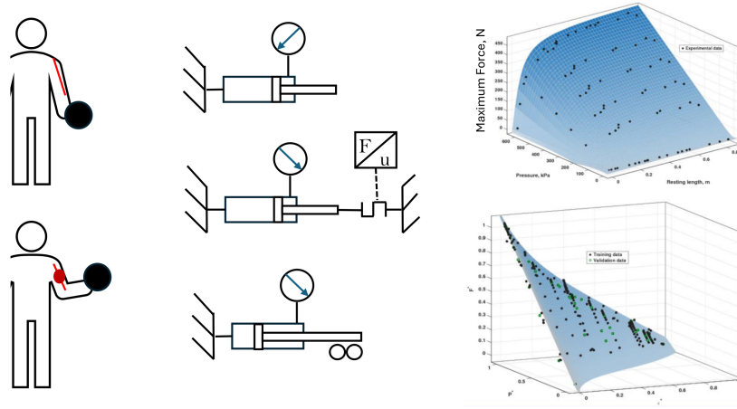
Figure 2.4: Overview of the BPA force-characterization study. Biological-muscle inspiration and the laboratory test apparatus lead to measured force-length–pressure data and fitted force surfaces used for actuator and robot design.
