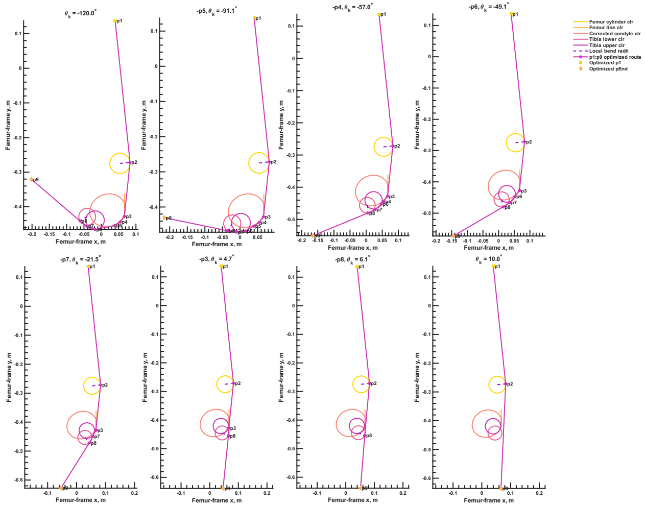
Figure C1: Eight-panel route-geometry view of the optimized 9-point extensor route of the 2026-09-25 design of record (Vas_Pam_20mm_Result_20260925.mat), drawn in the femur frame. Panels show full flexion ( \theta_k = -120.0^\circ ), the solver frame immediately before each contact-elimination event (before p5 at -91.1^\circ , p4 at -56.97^\circ , p6 at -49.09^\circ , p7 at -21.52^\circ , p3 at +4.75^\circ , and p8 at +6.06^\circ ), and full extension ( +10.0^\circ ); each interior panel title names the point released in the next frame. The circled polyline is the active p1:p9 route over the femur-cylinder, femur-wall, corrected-condyle, and tibia clearance envelopes; dashed lines mark the local bend radii at p2 and p8; the square marks the optimized origin p1 and the diamond the optimized distal endpoint pEnd. Regenerated by Export_AppendixRouteGeo.m, which ports the plotting block of Opt_run_Ext.m verbatim.
