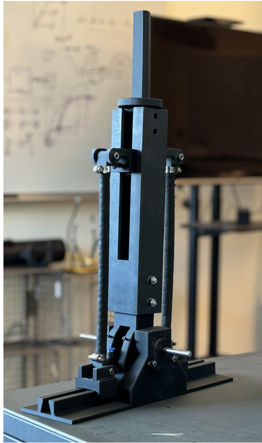
Figure 3.7: The BPA-actuated inverted-pendulum testbed. The pendulum shank rides on a hinge ankle above the foot assembly, and braided pneumatic actuators route down both sides of the shank to the foot, forming the antagonist ankle pair. Photograph from the AARL Inverted Pendulum project repository.
